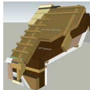
NBT Insulation Systems for Pitched Roof
